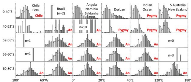
Fig. 2 All catches of blue whales in the Southern Hemisphere, including coastal and pelagic catches, and sexually immature and mature. The groupings by longitude and latitude are carefully chosen to divide the Southern Hemisphere into regions (of different sizes) with contrasting length frequencies. The large numbers of small blue whales in Angola, Namibia, and Saldanha are immature blue whales; sexually mature females were similar in size to those in the Antarctic regions. Where the three (possible) subspecies were clearly caught, these are indicated by An (Antarctic), Pygmy, or Chile. Shaded bars are longer than 80 ft (maximum recorded length of pygmy blue whales). Rounding to 5 ft intervals is visible in some regions, as is whale 'stretching' from 1937/38 when the minimum length of 70 ft was introduced. From the 2006 version of the IWC catch database.
