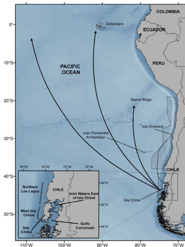
Fig. 4. Feeding ground of the Chilean blue whale, with inset showing summer survey areas off Isla de Chiloé and Golfo Corcovado. The hashed box shows the 1997 IDCRC-SOWER survey (Findlay In press), and black arrows show migratory linkages between Chiloé and lower latitude areas. A dotted line connects Isla de Chiloé and Isla Chañaral, representing a single whale re-sighted in both regions (Galletti Vernazzani et al. , In review) (2012).
