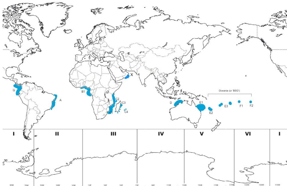
Fig. 2. Southern Hemisphere (A-G) and Northern Indian Ocean humpback whale (X) breeding stocks (blue) and high latitude Antarctic Areas (I-VI) where substantial modern whaling catches were made.
