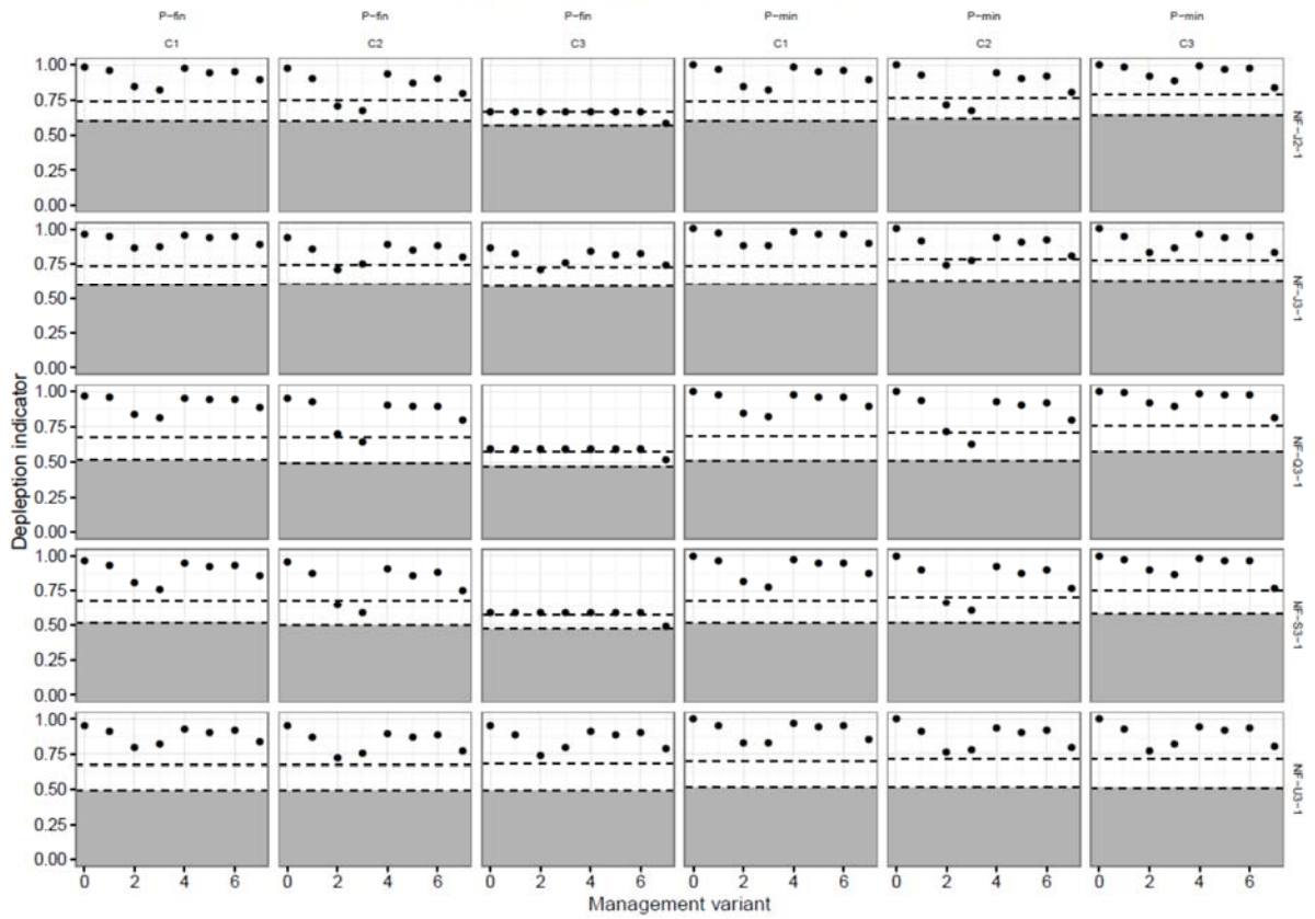
Fig. 3. A plot showing the performance of each RMP variant for each of the MSYR_{1+}=1\% trials. Results are presented for the C1, C2 and C3 sub-stocks and the two performance statistics on which the thresholds are based (P-fin: the lower 5th percentile of the final depletion distribution and P-min: the lower 5th percentile of the minimum depletion ratio distribution). The values for the performance statistics for each variant (and the no-catch scenario) are represented as dots, and horizontal lines indicate the thresholds (upper line: 'acceptable'; lower line: 'borderline'). The shaded area in this plot indicates 'unacceptable' performance.
