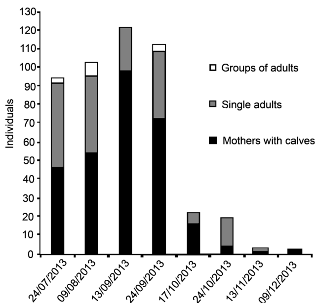
Fig. 3. Results of the 2013 season counts from the 'Punta Flecha' Observatory.
