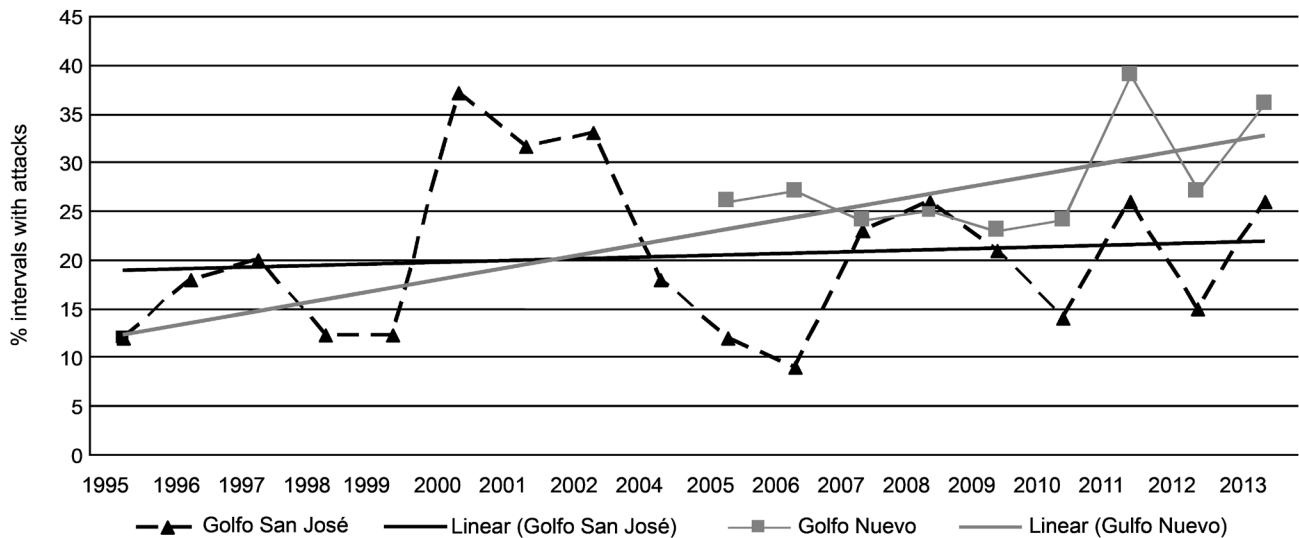
Fig. 6. Gull attack frequency in Golfo San José and Golfo Nuevo for the period 1995-2013.
