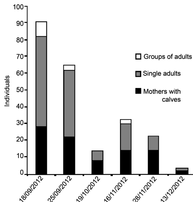
Fig. 2. Results of the 2012 season counts from the 'Punta Flecha' Observatory.
