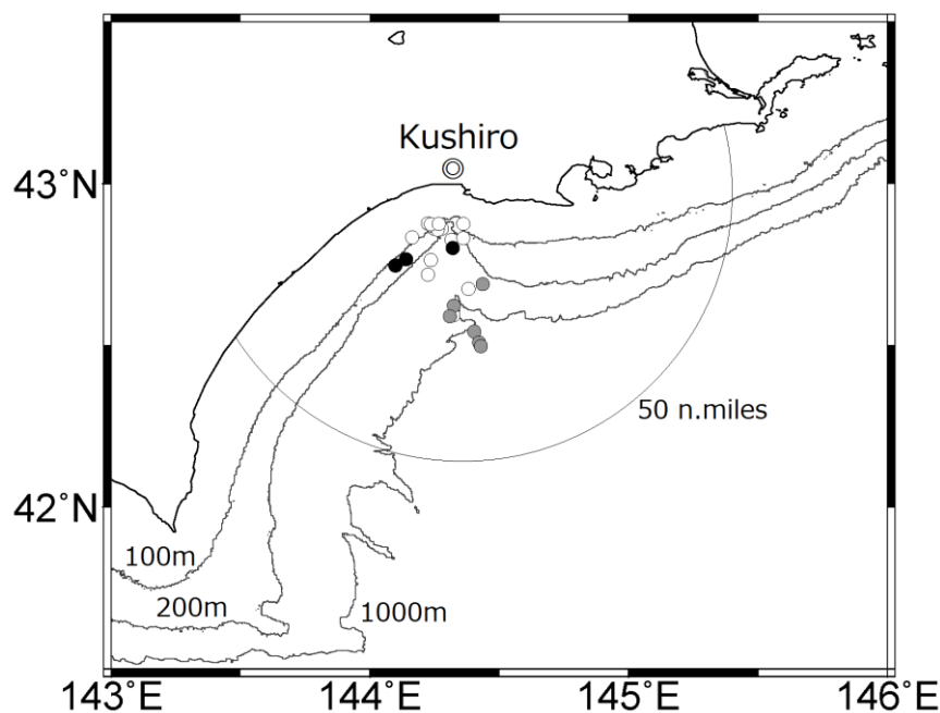
Figure 3. Sighting positions of humpback (white circle), fin (black) and sperm (gray) whales made by sampling vessels during the 2014 JARPN II coastal survey off Kushiro. Isobaths are 100m, 200m, and 1000m.
