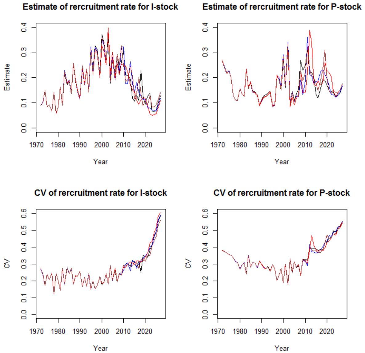
Fig. 5. Five replicated trajectories for estimates and CVs for the recruitment rate.
