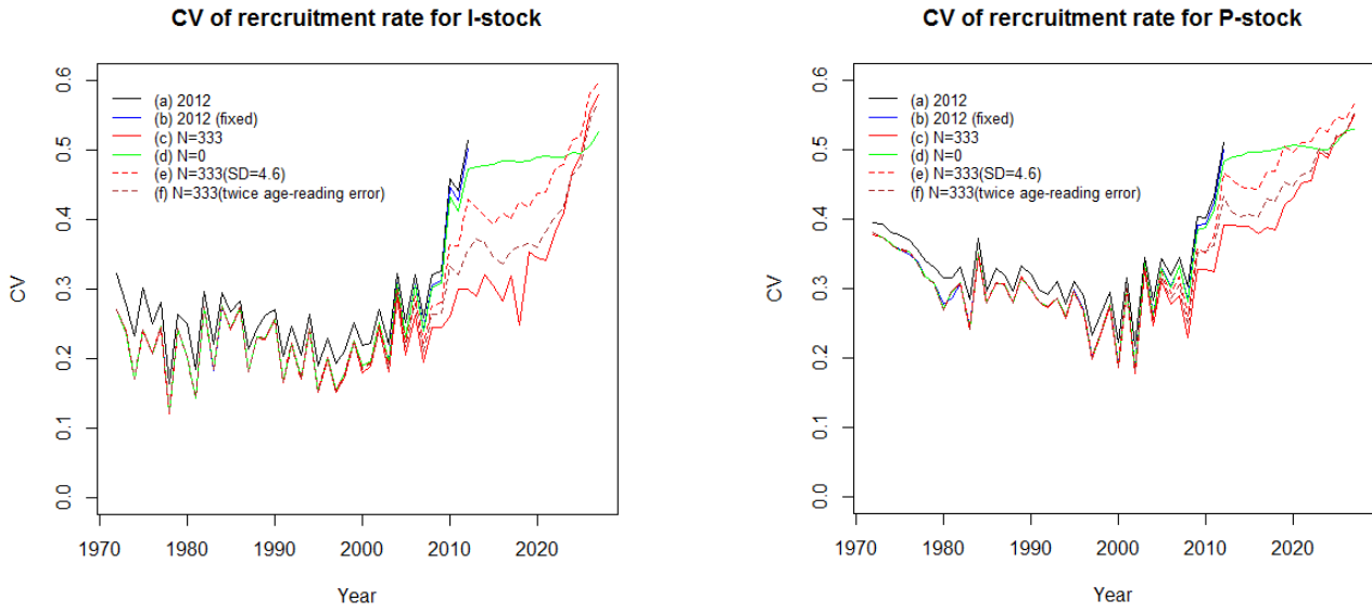
Fig. 3. Comparison of the trajectories of estimated CV for recruitment rates.
