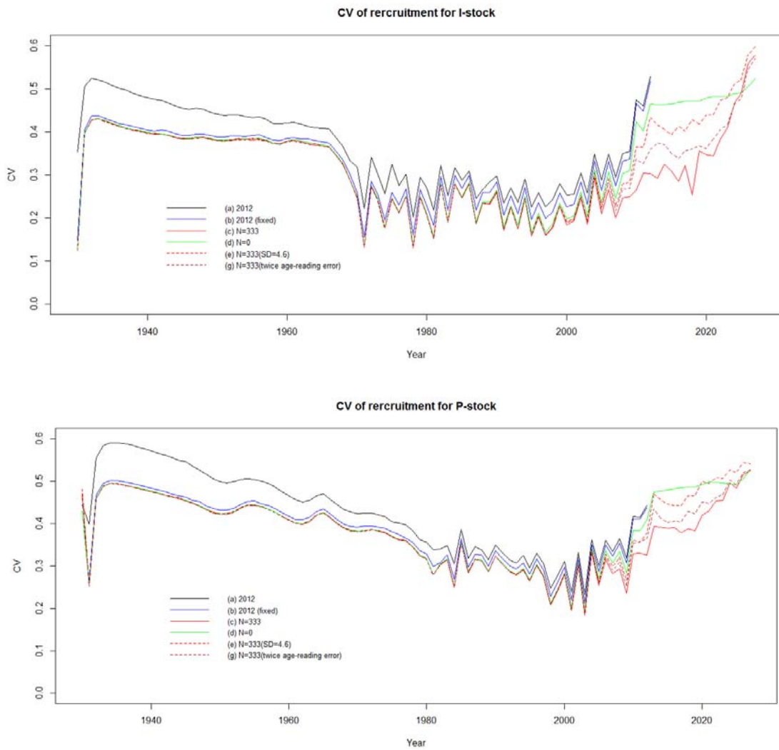
Fig. 4. Comparison of the trajectories of estimated CV for recruitment.
